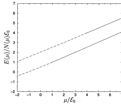
Fig. 2. Single-particle energy E/N as a function of the chemical potential \mu for the same states of Fig. 1. The solid and dashed lines are given by Eqs. (16) and (26), respectively.
