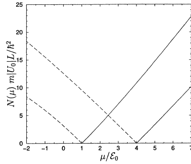
Fig. 1. Number of particles N as a function of the chemical potential \mu for the one dimensional square well. The solid and dashed lines are given by Eqs. (15) and (25), respectively. The two curves correspond to the states n=0 and n=1 .
