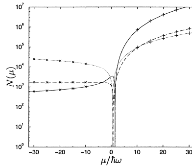
Fig. 5. Number of particles N as a function of the chemical potential \mu in the ground state of a quadratic potential with d=1 (dotted line), d=2 (dashed line) and d=3 (solid line). The symbols + and \times are the analytical results (36) and (43), respectively.
