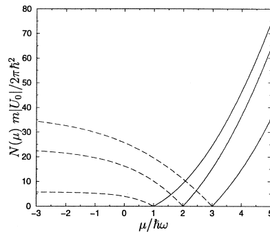
Fig. 3. Number of particles N as a function of the chemical potential \mu for a two dimensional quadratic potential. Solid and dashed lines are obtained by solving numerically Eq. (4) for U_0 > 0 and U_0 < 0 , respectively. The three curves correspond to the states (n, m) = (0, 0), (0, 1) and (1, 0) .
