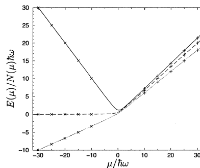
Fig. 6. Single-particle energy E/N as a function of \mu in the ground state of a quadratic potential with d=1 (dotted line), d=2 (dashed line) and d=3 (solid line). The dots + and \times are the analytical results (37) and (45), respectively.
