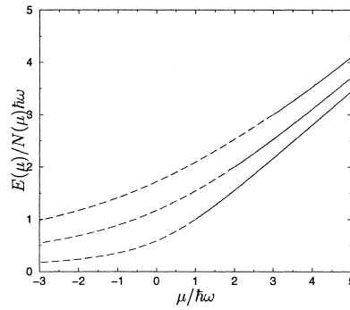
Fig. 4. Single-particle energy E/N as a function of the chemical potential \mu for the same states of Fig. 3.
